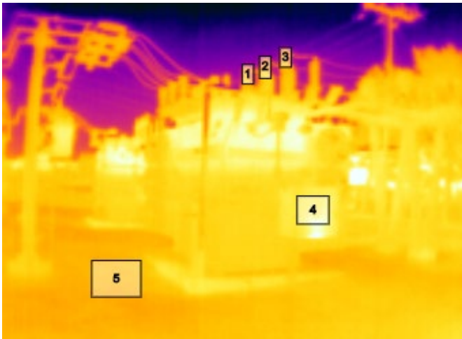
Figure 3 - Thermal snapshot of the transformer with boxes around the areas of interest where temperature will be measured.
